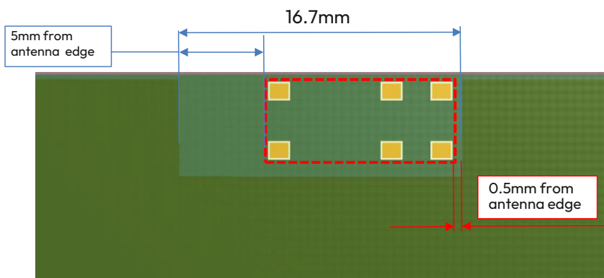
Centre PCB placement example
